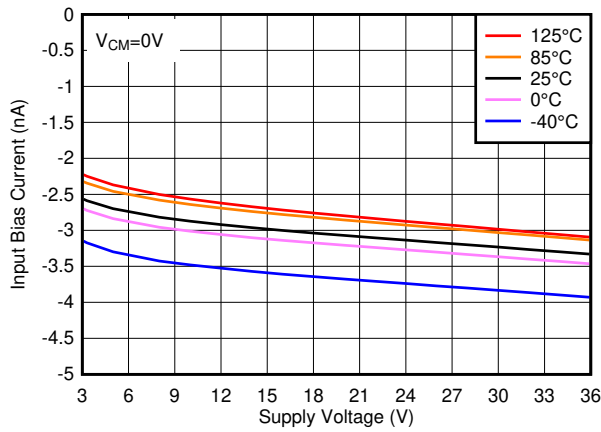
图 7-15. Input Bias Current vs. Supply Voltage
