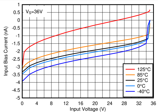
图 7-18. Input Bias Current vs. Input Voltage at 36V
