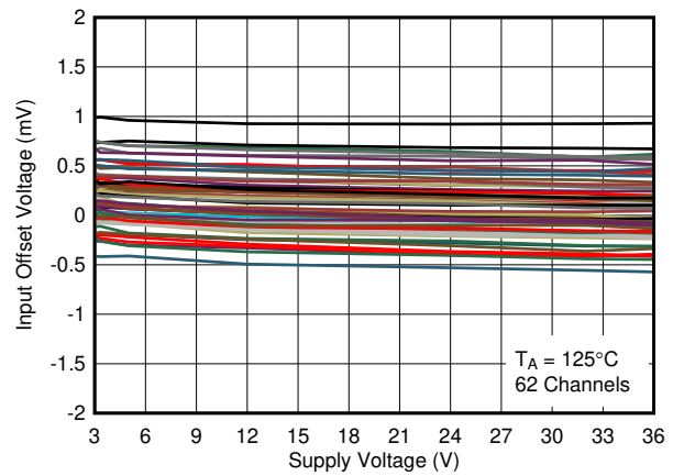
图 7-14. Input Offset Voltage vs. Supply Voltage at 125°C
