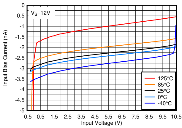
图 7-17. Input Bias Current vs. Input Voltage at 12V
