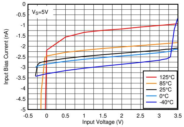
图 7-16. Input Bias Current vs. Input Voltage at 5V
